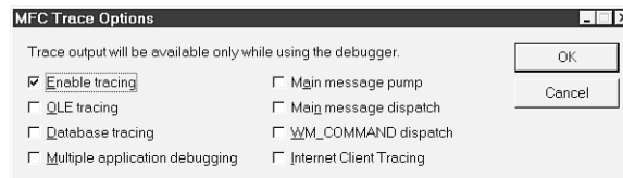
FIGURE E.16. The MFC Tracer tool options.
